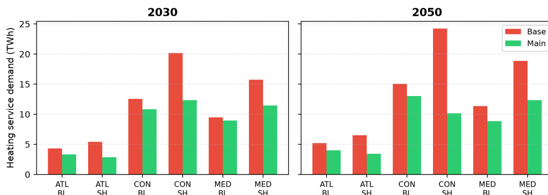
FIGURE 4, HEATING SERVICE DEMAND BY CLIMATE ZONE ( ATL , CON , MED ) AND BUILDING TYPE ( BL BLOCK , SH HOUSE ) IN 2030 AND 2050, BASE AND MAIN
