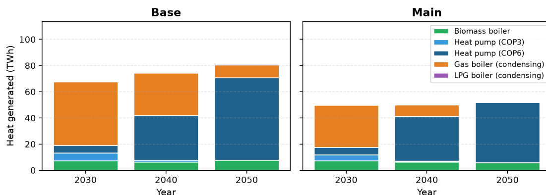
FIGURE 5, HEAT GENERATED BY TECHNOLOGY IN 2030, 2040 AND 2050, BASE AND MAIN (TWh). IN 2050 THE CONDENSING GAS BOILERS OF BASE BURN BIOMETHANE, NOT FOSSIL NATURAL GAS
